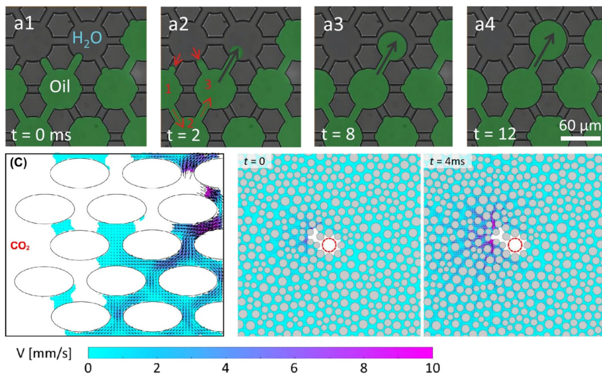
Fig. 26 [Top] High-speed images of a Haines jump event at Ca = 3.4 \times 10^{-6} . 196 [Bottom] Velocity vector fields during a Haines jump event in linear drainage and radial drainage. 146,167
