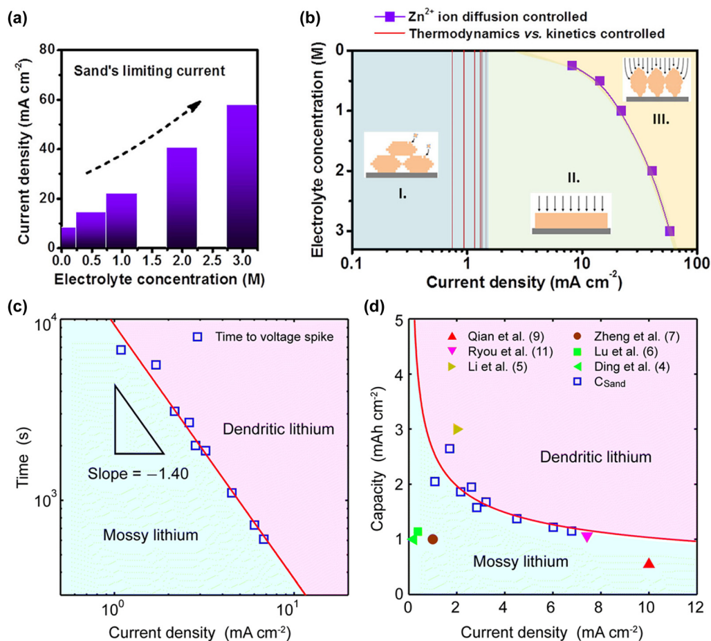
Fig. 73 (a) and (b) Sand's limiting current densities for Zn plating in aqueous \text{ZnSO}_4 electrolytes with different concentrations. The inset, model III, represents Zn dendrite growth. 811 (c) and (d) Sand's time and capacity for Li plating in nonaqueous Li electrolytes at various current densities. 812 Reprinted with permission from Angewandte Chemie International Edition (a) and (b) and Energy & Environmental Science (c) and (d).
