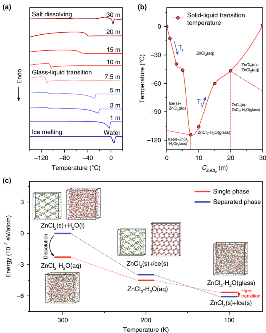
Fig. 49 (a) Differential scanning calorimetry curves and (b) obtained phase transition diagram of a \text{ZnCl}_2/\text{water} binary system. (c) Calculated transition state in the transformation from the glass state to the separated crystalline state of a 7.5 m \text{ZnCl}_2/\text{H}_2\text{O} solution. 585 Reprinted with permission from Nature Communications .
