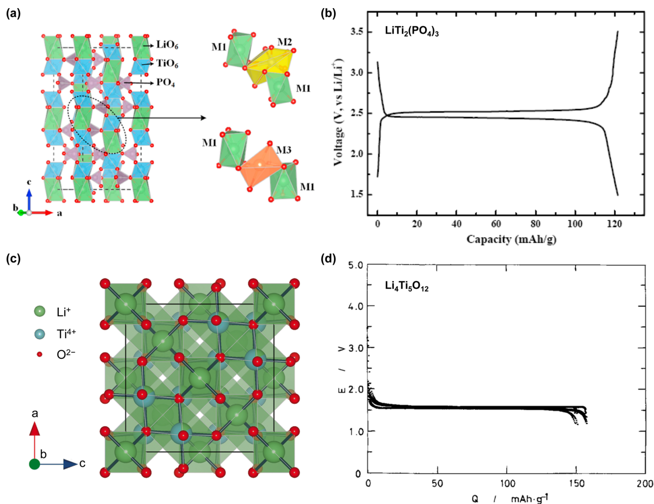
Fig. 26 Crystal structures and electrochemical properties of (a) and (b) \text{LiTi}_2(\text{PO}_4)_3 . 60,301 and (c) and (d) \text{Li}_4\text{Ti}_5\text{O}_{12} . 302,303 Lithiation/delithiation curves of \text{LiTi}_2(\text{PO}_4)_3 and \text{Li}_4\text{Ti}_5\text{O}_{12} were obtained in 1 M \text{LiPF}_6 /ethylene carbonate : dimethyl carbonate : ethyl methyl carbonate (1 : 1 : 1, v : v : v) and 1 M \text{LiClO}_4 /ethylene carbonate : 1,2-dimethoxyethane (1 : 1, v : v), respectively. Reprinted with permission from Energy Storage Materials (a), Advanced Functional Materials (b), Advanced Composites and Hybrid Materials (c), and Journal of The Electrochemical Society (d).
