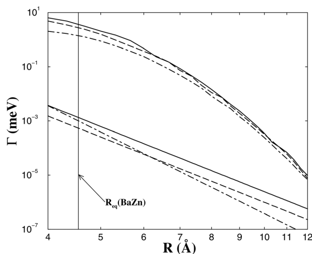
Fig. 1 Total ICD rates of BaZn resulting from Zn 3d sub-shell ionization as a function of the internuclear distance R . The vertical line indicates the equilibrium distance R eq of the BaZn dimer. The three upper curves show the ab initio calculated results for \Gamma_0 , \Gamma_{\pm 1} , and \Gamma_{\pm 2} . The three lower curves show the quadrupole–dipole ( \Gamma_0 , \Gamma_{\pm 1} ) and the quadrupole–quadrupole ( \Gamma_{\pm 2} ) asymptotic approximations resulting from the Coulomb interaction (see text). Solid lines: 3d 0 vacancy; dashed lines: 3d ±1 vacancy; dash-dot lines: 3d ±2 vacancy. Reproduced with permission from the American Physical Society, ref. 47, Copyright 2004.
