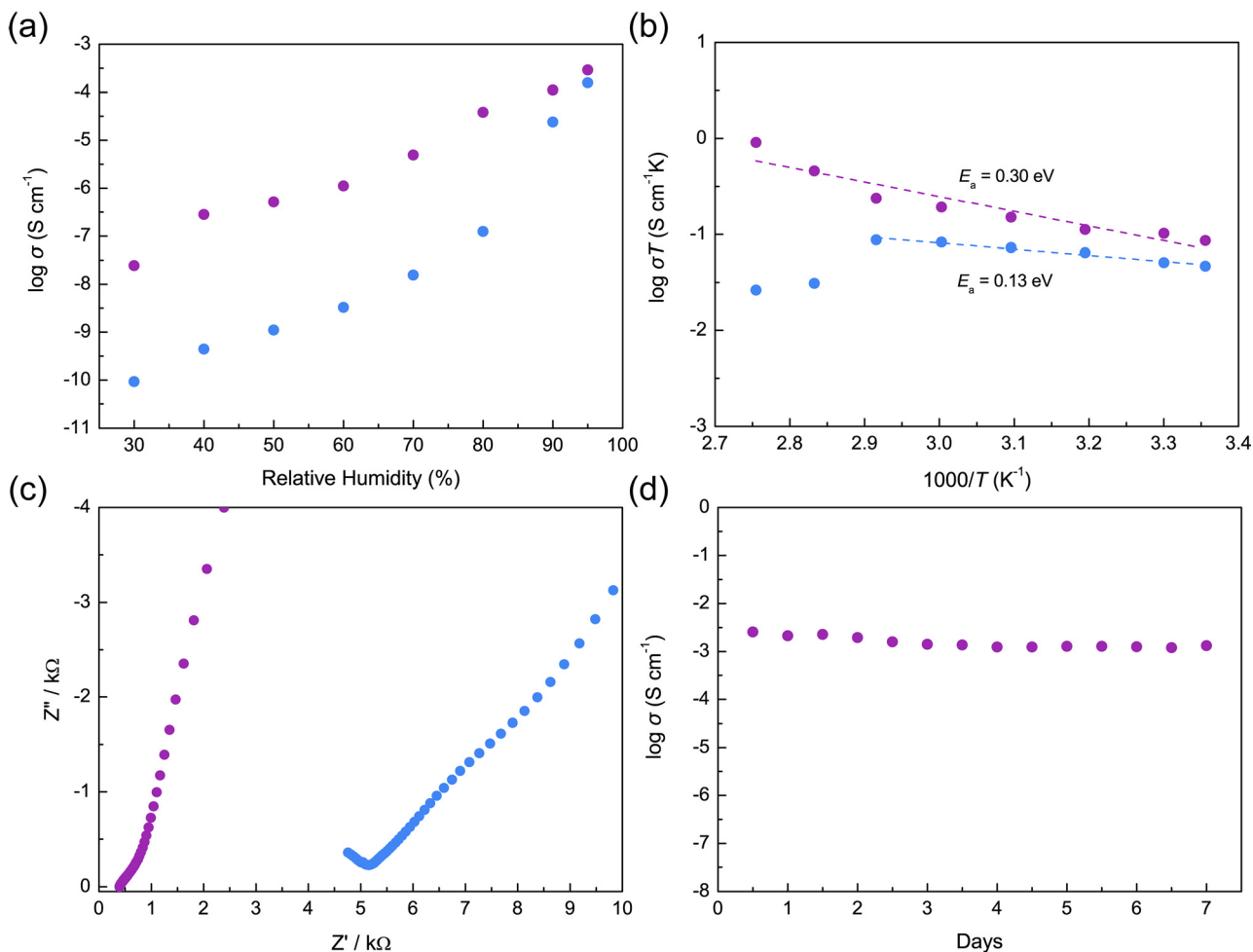
Fig. 4 (a) Humidity-dependent conductivity of Y-DSNDC (blue) and K-DSNDC (purple) measured at 298 K. (b) Arrhenius plots for Y-DSNDC (blue) and K-DSNDC (purple) in the temperature range of 298–363 K under 95% RH. (c) Nyquist plots of the highest conductivity for Y-DSNDC (blue) and K-DSNDC (purple) measured at 343 K and 363 K under 95% RH, respectively. (d) Long-term stability of the proton conductivity for K-DSNDC at 363 K under 95% RH.
