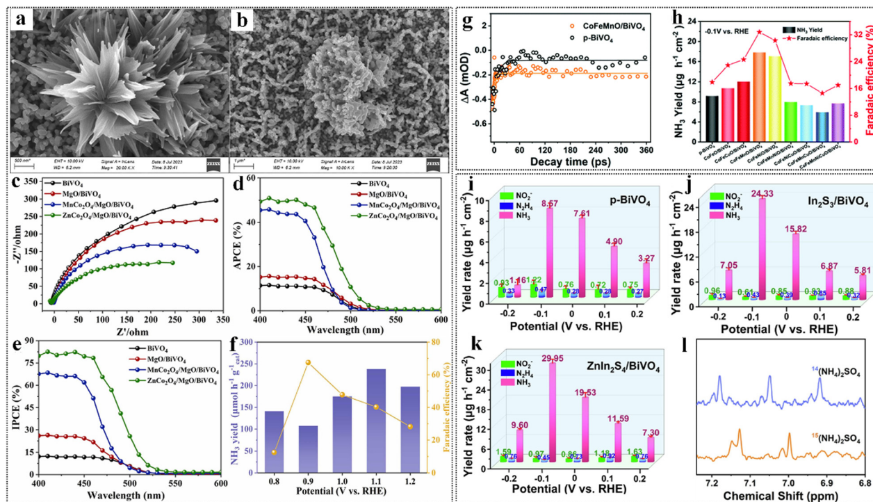
Fig. 5 (a) SEM images of \text{MnCo}_2\text{O}_4/\text{MgO}/\text{BiVO}_4 and (b) \text{ZnCo}_2\text{O}_4/\text{MgO}/\text{BiVO}_4 . (c) EIS, (d) APCE and (e) IPCE diagrams of \text{BiVO}_4 , \text{MgO}/\text{BiVO}_4 , \text{MnCo}_2\text{O}_4/\text{BiVO}_4 ( M = \text{Zn}, \text{Mn} ) and \text{MnCo}_2\text{O}_4/\text{MgO}/\text{BiVO}_4 ( M = \text{Zn}, \text{Mn} ). (f) Ammonia formation rates (the average value on 2 h reaction) and corresponding faradaic efficiencies of \text{ZnCo}_2\text{O}_4/\text{MgO}/\text{BiVO}_4 . Reproduced from ref. 120 with permission from Elsevier, copyright 2024. (g) Characteristic dynamics of p\text{-BiVO}_4 and \text{CoFeMnO}/\text{BiVO}_4 probed at 480 nm. (h) Yield of \text{NH}_3 and faradaic efficiency ( A\text{-M}_x\text{O}_y/p\text{-BiVO}_4 ) at -0.1\text{ V} vs. RHE. Reproduced from ref. 121 with permission from Royal Society of Chemistry, copyright 2022. Yield rates of (i) p\text{-BiVO}_4 , (j) \text{In}_2\text{S}_3/\text{BiVO}_4 and (k) \text{ZnIn}_2\text{S}_4/\text{BiVO}_4 under different voltages. (l) Qualitative experiments of ^{14}\text{NO}_3^- and ^{15}\text{NO}_3^- isotopes. Reproduced from ref. 122 with permission from Elsevier, copyright 2022.
