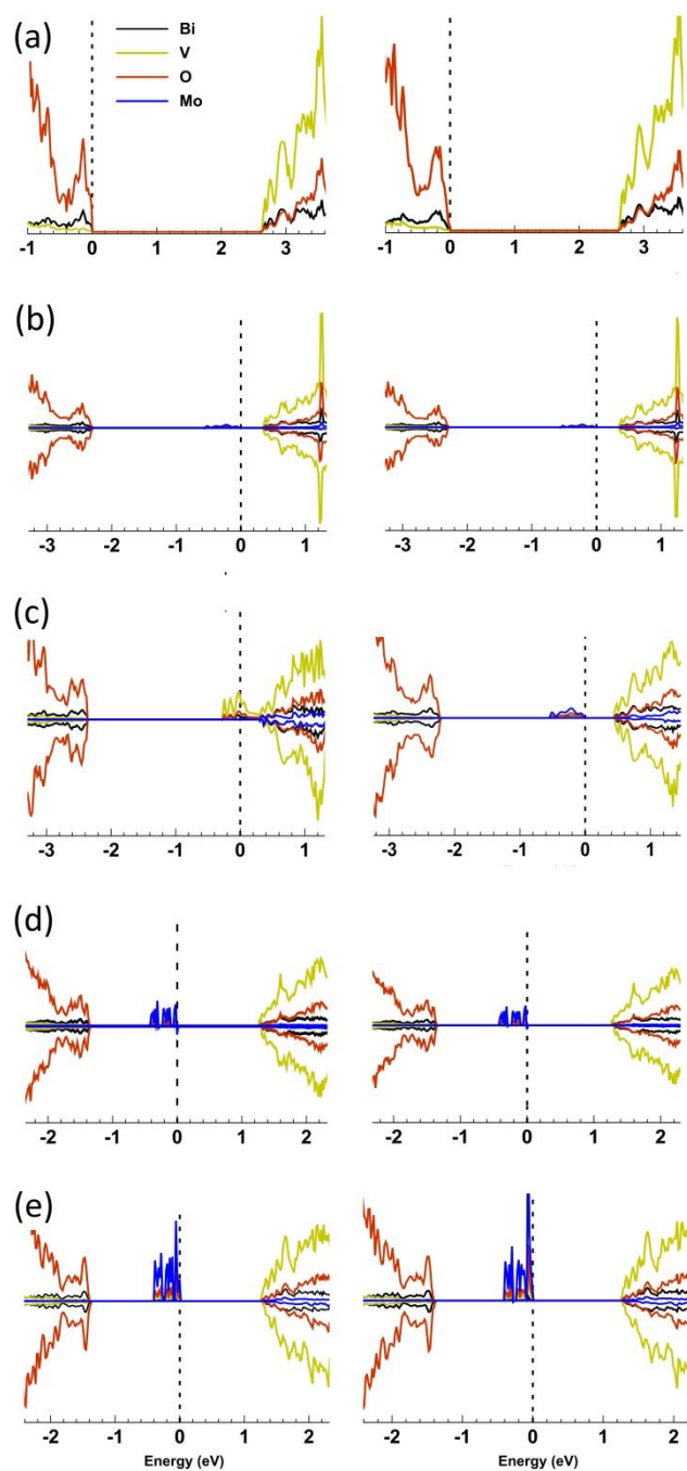
Figure 11: Comparison of the PDOS for (left) t-BiVO 4 and (right) m-BiVO 4 host structures for (a) undoped, (b) 6.25 at.% Mo in a V site, (c) 12.5 at.% Mo in a V site, (d) 6.25 at.% Mo in a Bi site, and (e) 12.5 at.% Mo in a Bi site. For each host structure, the VBM, formed primarily by O orbitals, are plot at the same position to one another. The PDOS are drawn for energies \sim 1 eV below the VBM up to \sim 1 eV above the CBM, which is formed primarily by V orbitals. The dashed line represents the highest occupied state in each structure.
