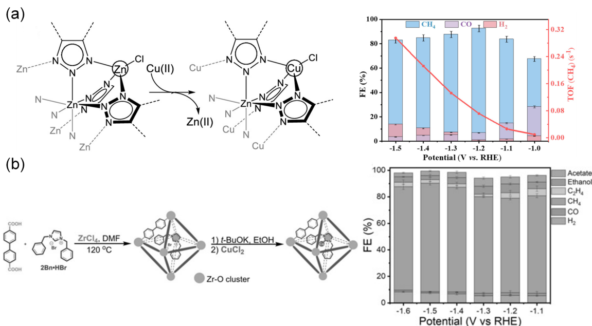
Fig. 6 (a) Schematic of the metal transformation process, and \text{FE}_{\text{CH}_4} and TOF of \text{Cu}_4\text{I-MFU-4l} . 121 Copyright 2021, American Chemical Society. (b) Schematic synthesis route and FE of 2Bn-Cu@UiO-67. 120 Copyright 2021, Wiley-VCH.
