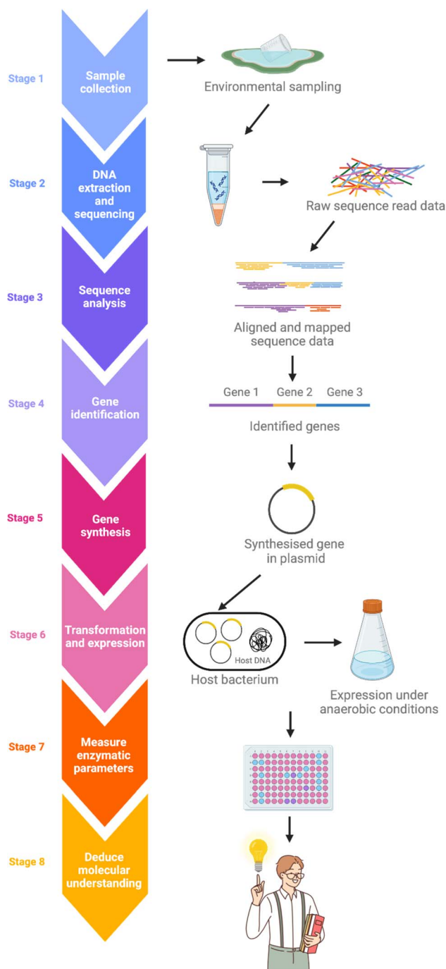
Fig. 5 Schematic of a typical metagenomics workflow. DNA is extracted from selected samples and sequenced. The raw sequence data is analysed, and the genes of interest are identified, allowing for their synthesis, transformation and expression under the required laboratory conditions. The workflow leads to further experimental procedures for enzymatic molecular understanding. Created with https://BioRender.com .
