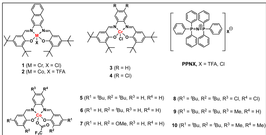
Fig. 1 Different \text{M}(\text{Salophen})\text{X} ( \text{M} = \text{Co} , \text{Cr} ) metal complexes.
