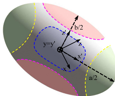
Fig. 11 The final steady-state shape of droplet/capsule with the major axis, a , the minor axis of deformation, b , and the third axis, c . An additional reference frame (x', y', z') is defined, with the axes corresponding to the deformed droplet principal axes. The different regions of the droplet have been also highlighted for ease of reference: tips (green), belly (red) and sides (blue). Inspired by ref. 169.
