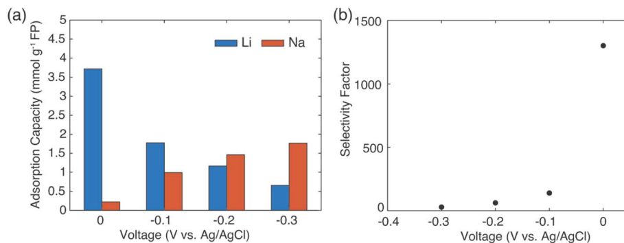
Fig. 9 Electrochemical reduction of FP to capture cations from a brine solution containing \text{Li}^+ : \text{Na}^+ molar ratio of 1 : 78. (a) The cations adsorption capacity of the working electrode (FP) and (b) the selectivity factor \alpha_{\text{Na}}^{\text{Li}} for FP was assessed after 50% extent of reduction of the FP at constant voltages of 0, -0.1, -0.2, and -0.3 V (vs. Ag/AgCl).
