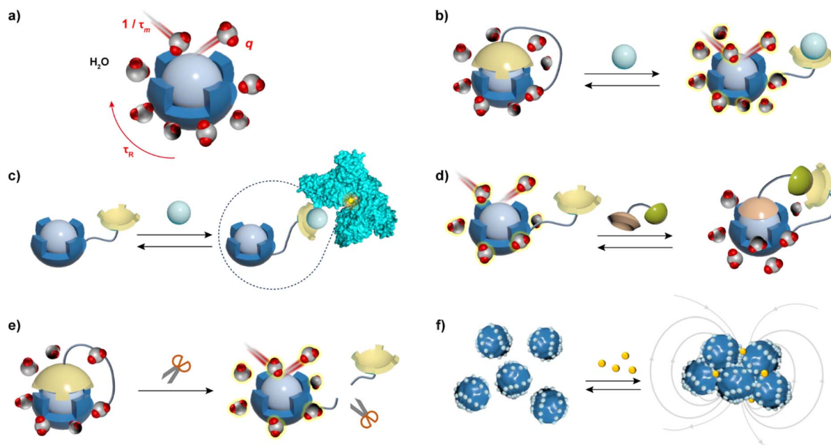
Fig. 1 Main parameters that influence r_1 and r_2 , and typical mechanisms that cause their changes in T_1 and T_2 bioresponsive MRI CAs. (a) Typical T_1 agents are paramagnetic metal ion complexes and the key parameters that influence their r_1 are: hydration number ( q ), mean residence time of bound water ( \tau_m ) and rotational correlation time ( \tau_R ) of the complex. (b) The recognition unit (yellow cap) of the responsive CA interacts with the target analyte (e.g. biologically relevant metal ions); the switch of recognition unit concurrently changes the q and r_1 values of the CA. (c) The recognition unit on the responsive CA interacts with the target analyte, but also forms ternary complexes with large molecules, such as proteins. This leads to a decrease in \tau_R due to formation of the high molecular weight species, which increases r_1 at low-to-intermediate magnetic fields. (d) The fixed geometry and functional groups of the responsive CA interact with ditopic guests, such as zwitterionic amino acid neurotransmitters. In the absence of the analyte, water is coordinated to the paramagnetic metal ion. In the presence of the ditopic guest molecule, the formation of the ternary complex with the responsive CA decreases q , and hence the r_1 . (e) The enzyme activity causes the removal of functional and paramagnetic ion-coordinating group from the responsive CA, which results in increases of the q and r_1 values. (f) Typical T_2 CAs are composed of superparamagnetic nanoparticles with target-specific coatings on the surface. In the presence of the target analyte, the interaction between functional surfaces typically induces the aggregation of nanoparticles, which affects the \tau_R of the agent and diffusion of water on the responsive CA surface, resulting in strong r_2 changes. The processes described here lead to (b), (c), (e), (f) increase, and (d) decrease of the MRI signal.
