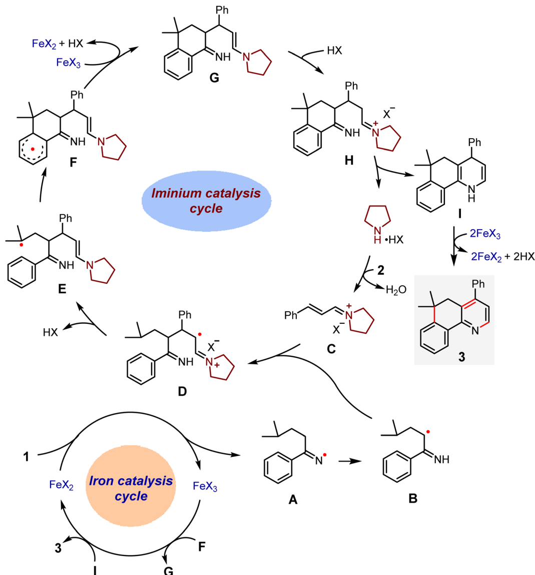
Scheme 7 Proposed mechanism for the relay annulation via synergistic iron and iminium catalysis ( X = \text{ClO}_4 , OBz, or acac).
