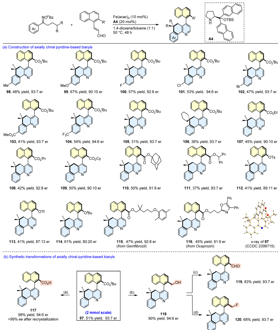
Scheme 9 (a) Construction of axially chiral pyridine-based biaryls. Reaction conditions: oxime ester (0.6 mmol), enal (0.2 mmol), \text{Fe}(\text{acac})_3 (10 mol%), A4 (20 mol%), 1,4-dioxane/toluene (2 mL, v/v = 1/1), 50 °C, 48 h, under \text{N}_2 . (b) Synthetic transformations of 97 . Reaction conditions: (a) NaOH (2 M), 95% EtOH, 100 °C, 24 h. (b) DIBAL-H (2.5 equiv.), DCM, −78 °C, 2 h. (c) IBX (1.2 equiv.), HOAc (1.2 equiv.), MeCN, rt, 6 h. (d) DAST (4 equiv.), DCM, 0 °C to rt, 12 h.
