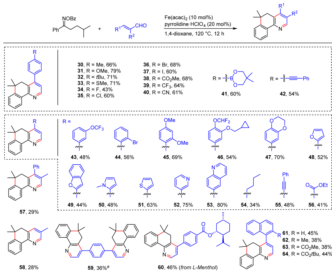
Scheme 4 Substrate scope of enals. Reaction conditions: oxime ester (0.6 mmol), enal (0.2 mmol), \text{Fe}(\text{acac})_2 (10 mol%), pyrrolidine·HClO 4 (20 mol%), 1,4-dioxane (2 mL), 120 °C, 12 h, under N 2 . a Oxime ester (1.2 mmol), cinnamaldehyde (0.2 mmol), \text{Fe}(\text{acac})_2 (20 mol%), pyrrolidine·HClO 4 (40 mol%), 1,4-dioxane (4 mL), 120 °C, 12 h, under N 2 .
