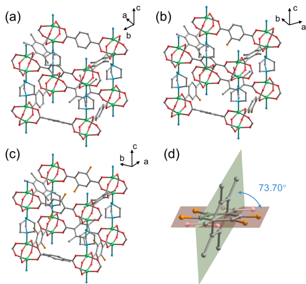
Fig. 1 Expanded cubic-like structure of (a) DMOF-0F , (b) DMOF-1F , and (c) DMOF-2F , in which only one orientation of the disordered xFBDC ligand is shown. (d) Disorder of 1FBD and 2FBD in DMOF-1F . Hydrogen atoms are omitted for clarity. Colour code: C: grey; F: orange; N: blue; O: red; Zn: green.
