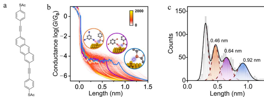
Fig. 12 (a) Structure of 2,6-bis((4-acetylthio)phenyl)ethynyl anthracene with acetyl-protected thiol(ate) ( -S_{Ac} ) terminal groups; (b) 2D conductance–displacement histograms for the junctions in TIB/TCB. The orange/purple/blue lines are three typical single traces with different plateau lengths. Insets: schematic illustration of Au–S bonds in different cases: interaction with I (orange), with Cl (purple), and without I or Cl (blue); (c) conductance plateau lengths for junctions in TIB/TCB: the blue colour represents the parent junctions, the purple colour represents the case with Cl \cdots Au interactions, the orange colour represents the case with I \cdots Au interactions. Figures adapted with permission from ref. 130. Copyright 2023, Springer Nature.
