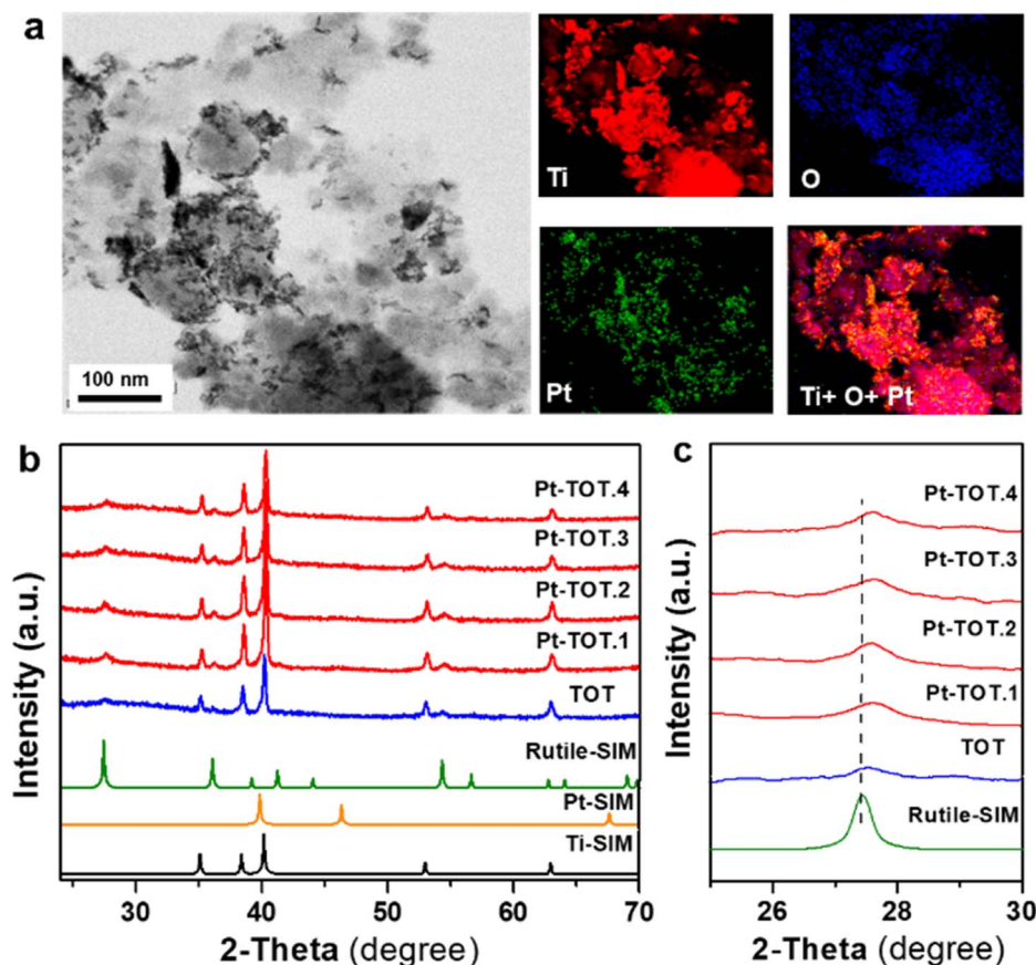
Fig. 1 (a) STEM and EDS elemental mapping of Pt-TOT.2, (b) XRD pattern, and (c) expanded XRD pattern from 2\theta = 24 to 30^\circ of TOT and Pt-TOTs with different Pt content (the dashed line shows the diffraction peak position of rutile \text{TiO}_2 ).
