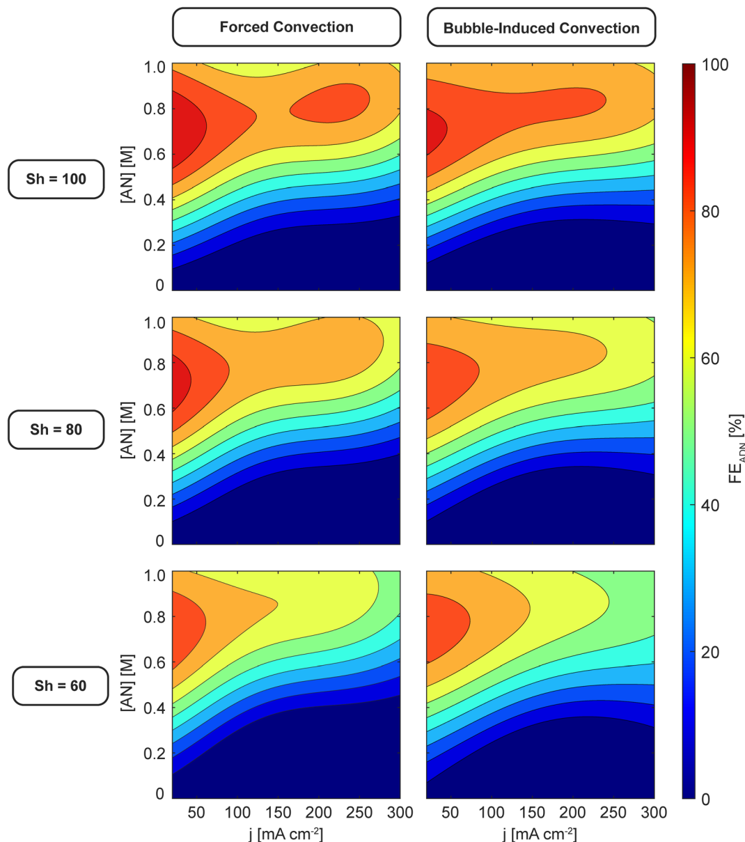
Fig. 6 2D slices of the 3D surrogate models at different mass transport conditions: Sh = 60 , 80 , and 100 for forced convection (left column) and bubble-induced convection (right column). All plots present predicted values from the surrogate models built on experimental data. The experiments were conducted at ambient temperature and pressure. In addition to AN, the electrolyte contained 0.5 M Na_3PO_4 , 0.03 M EDTA, and 0.02 M TBA hydroxide.
