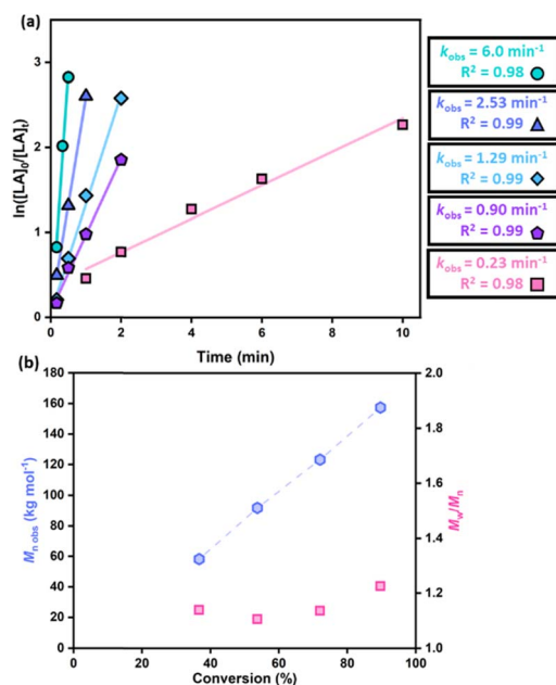
Fig. 2 (a) Semi-logarithmic plot of rac -LA conversion vs. time at 70 °C with Zn(OBn)_2 in toluene solvent with various [cat] : [ rac -LA] loading ratios ( [rac-LA] = 1 \text{ M} for 1 : 100 (circles); 1 : 300 (triangles); 1 : 500 (diamonds) and 1 : 1000 (pentagon) loadings, and 2 M for 1 : 2500 (square) loadings, with k_{obs} and R^2 values presented in the figure legend. (b) Evolution in M_n and M_w/M_n with monomer conversion for a [Zn(OBn)_2] : [rac-LA] ratio of 1 : 2500 ( [rac-LA] = 2 \text{ M} ) (refer to ESI, Fig. S4,† for additional plots of M_n vs. M_w/M_n ).
