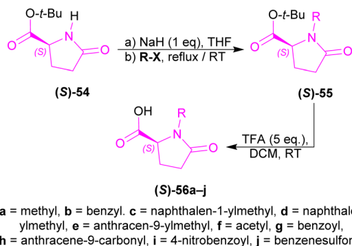
Scheme 15 Synthesis of (S)-pyroglutamic acid derivatives.
