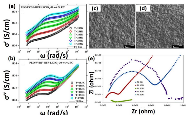
Fig. 5 (a) Real and (b) imaginary plots of conductivity for PEO/PVDF-HFP-LiClO 4 -30 wt% ECs, FE-SEM images of (c) PEO/PVDF-HFP-LiClO 4 -30 wt% PCs, (d) PEO/PVDF-HFP-LiClO 4 -30 wt% DMCs polymer solid electrolytes. 94 Reproduced ref. 94 with permission from American Chemical Society, Copyright 2017, (e) impedance plot of PCL/LiCF 3 SO 3 and PC plasticizer with different composition. 95 Reproduced ref. 95 with permission from Institute of Physics, Copyright 2020.
