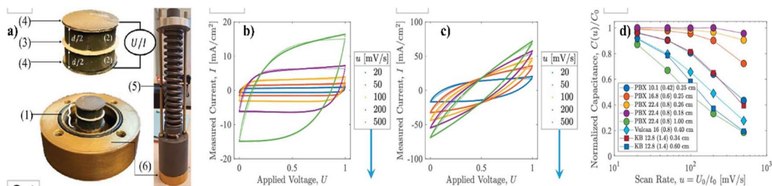
Fig. 7 (a) (1) An electric double-layer capacitor (EDLC) composed of (2) two polished, electrolyte-saturated carbon–cement electrodes (thicknesses) d separated by (3) a glassy fiber membrane soaked in the same electrolyte (1 M KCl) and covered by (4) conductive graphite paper. The electrodes are (5) prestressed in (6) a closed cell to improve contact between the charge collectors and the electrodes. (b and c) Steady-state CV measurements of current, I , during cyclic charge/discharge at different scan rates, u = U_0/t_0 , for two carbon–cement electrode samples prepared with different carbon blacks, water-to-cement ratios, and electrode thicknesses. (d) By applying eight different carbon–cement electrode materials with different carbon black materials, mix designs, and electrode thicknesses, a characteristic scaling of the rate-dependent CV capacitance is obtained, which is indicative of the high rate capability of the electrode materials. Reproduced from ref. 6 with permission from PNAS, copyright 2024.
