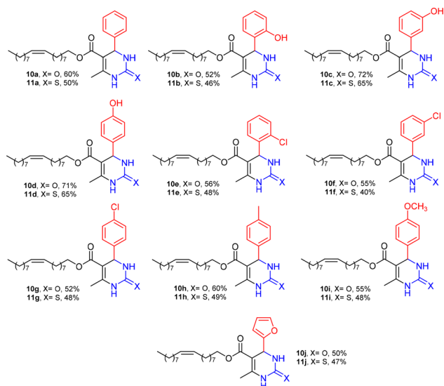
Fig. 2 Fatty chain 5-substituted DHPMs from Biginelli's MCR.
