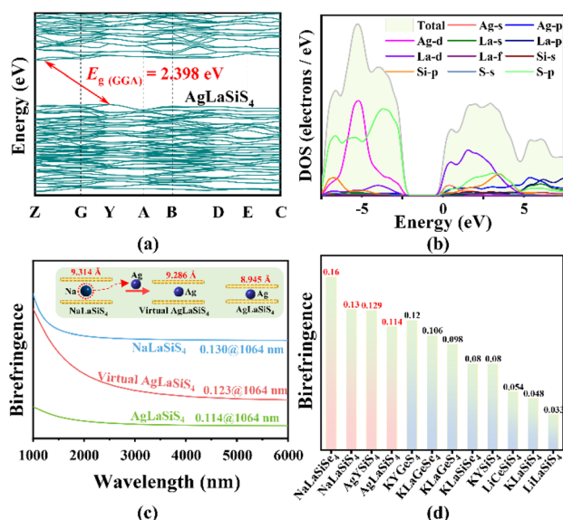
Fig. 5 The band structures (a) and the T/ PDOS (b) of \text{AgLaSiS}_4 ; (c) the calculated birefringence of \text{AgLaSiS}_4 , virtual \text{AgLaSiS}_4 , and \text{NaLaSiS}_4 (inset diagrams show the fluctuation of layer distance in \text{AgLaSiS}_4 , \text{NaLaSiS}_4 and virtual \text{AgLaSiS}_4 built from \text{NaLaSiS}_4 ); (d) statistical birefringence (at 1064 nm) of title compounds and other compounds in the \text{A}^{\text{I}}\text{RE}^{\text{III}}\text{C}^{\text{IV}}\text{Q}_4^{\text{VI}} family.
