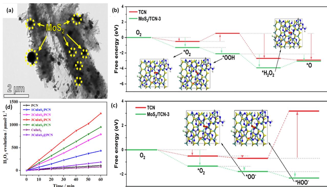
Fig. 27 (a) SEM images of \text{MoS}_2 - \text{TCN-3} . Free energy change graphs for the \cdot\text{HO}_2^- 2e^- ORR pathway under (b) acidic and (c) alkaline conditions. The figures are adapted with permission from ref. 201. Copyright 2023, Elsevier. (d) Photocatalytic \text{H}_2\text{O}_2 generation by PCN, \text{CuInS}_2 , 3\text{CuInS}_2 @PCN, and x\text{CuInS}_2 /PCN samples. The figures are adapted with permission from ref. 202. Copyright 2023, Elsevier.
