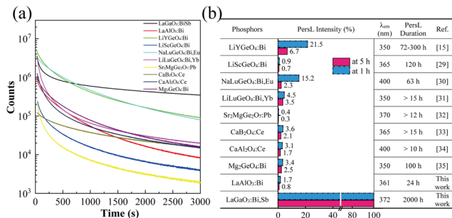
Fig. 7 (a) PersL decay curves of several ultra-long UVA PersL reported phosphors measured at 60 s after 10 min of X-ray irradiation. (b) Comparison of PersL intensity of different UVA PersL phosphors 1 h and 5 h after 10 min of X-ray excitation. The PersL intensity was normalized by LaGaO 3 :Bi,Sb at 1 h and 5 h. Note that the PersL duration of other UVA PersL materials was extracted from references.
