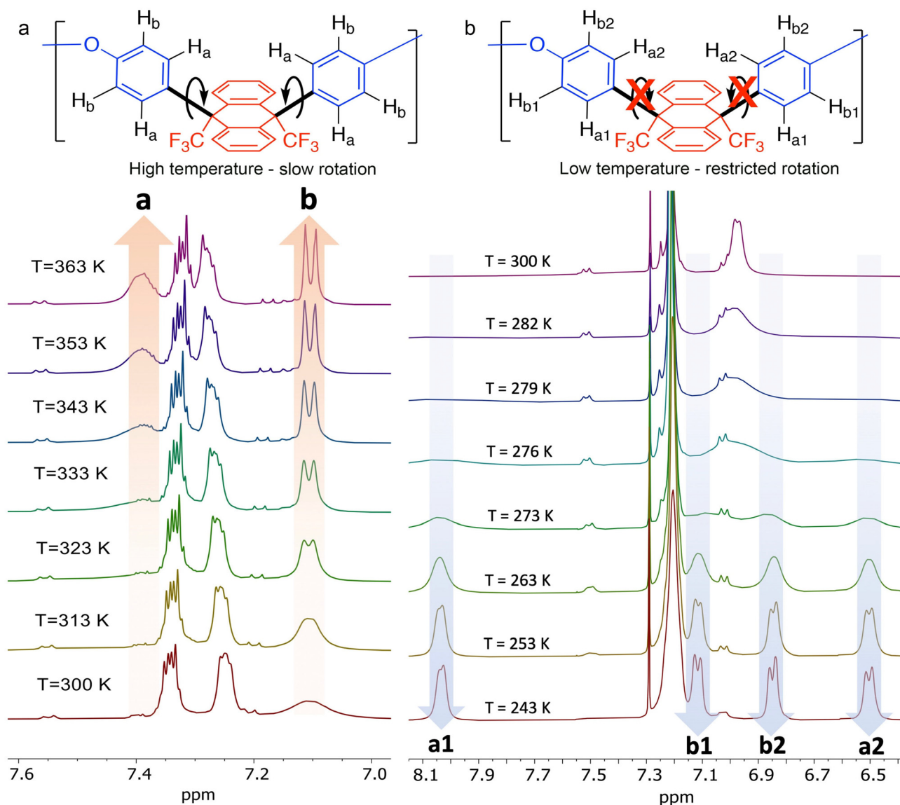
Fig. 3 Variable temperature NMR of polymer BTFMA-DPE acquired in the ranges (a) 300–363 K (in DMF- d_7 ) and (b) 243–300 K (in CDCl _3 ). Due to hindered rotation of the benzene rings of the DE monomeric unit, the peak for the hydrogens ( H_a ) adjacent to the new bond only becomes distinct at higher temperatures. At lower temperatures, rotation is frozen so that each of the protons H_{a1} , H_{a2} , H_{b1} and H_{b2} show a distinct peak.
