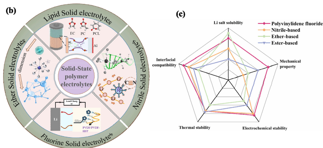
Fig. 1 Schematic illustration of a battery. (a) \text{Li}^+ transport in polymer electrolytes and growth of lithium dendrites, (b) typical polymer electrolytes, (c) Radar map of properties of different polymers.
