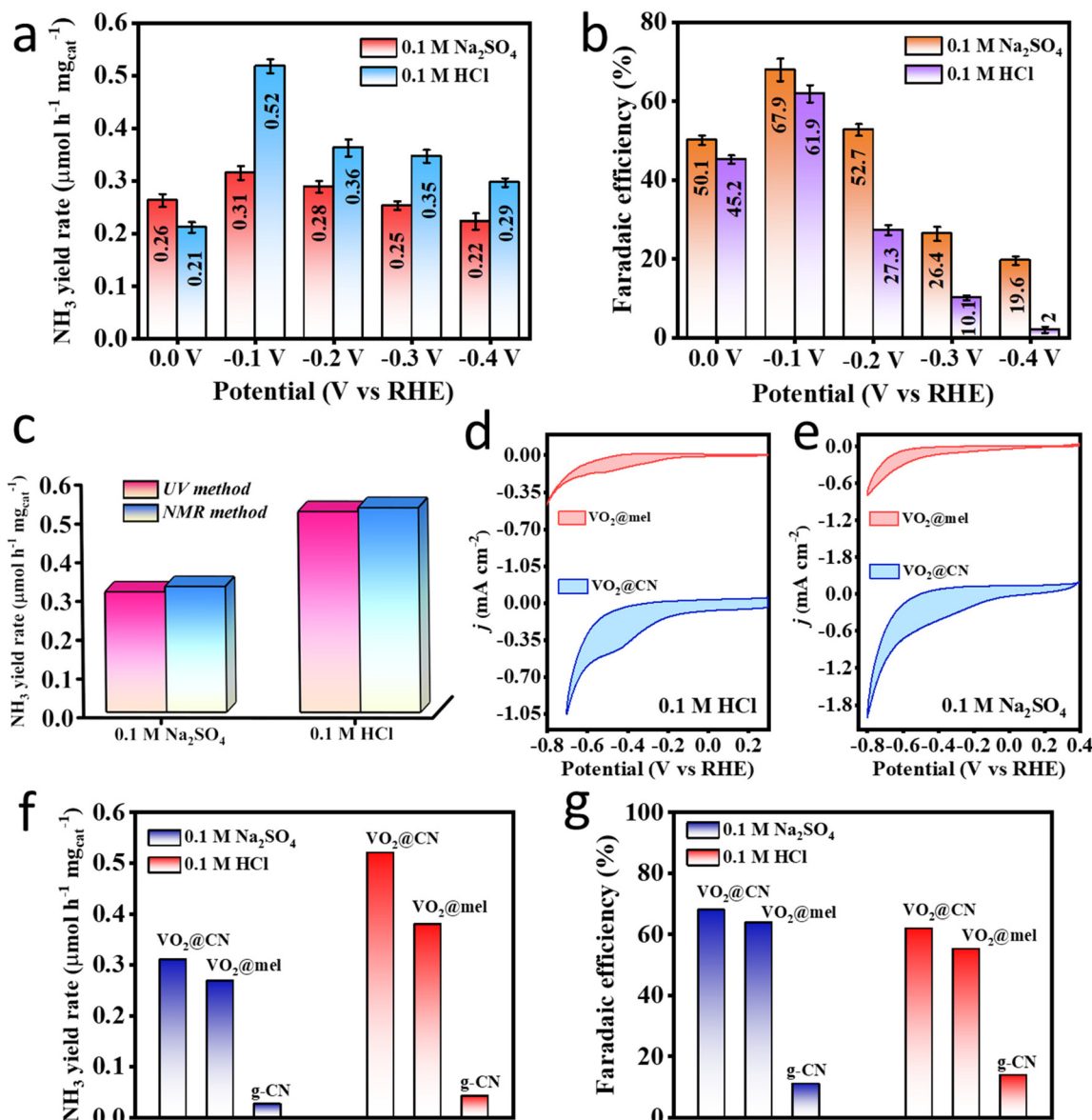
Fig. 4 NRR performance comparison of the VO 2 @CN catalyst in both 0.1 M Na 2 SO 4 and 0.1 M HCl electrolytes. (a and b) NH 3 yield rate and FE of the catalyst over the wide-ranging potential window from 0.0 V to -0.4 V vs. RHE in the presence of continuous N 2 purging; (c) quantitative analyses of NRR performance of VO 2 @CN using UV-visible and NMR methods; CV curves of VO 2 @CN and VO 2 @mel samples in (d) 0.1 M HCl and (e) 0.1 M Na 2 SO 4 showing an enhancement in the current density upon graphitization of melamine due to increased conductivity; (f) NH 3 yield rate and (g) FE comparison of VO 2 @CN with control samples like VO 2 @mel and g-CN in both acidic and neutral electrolyte media. The error bars represent the standard deviation values for three different data-sets.
