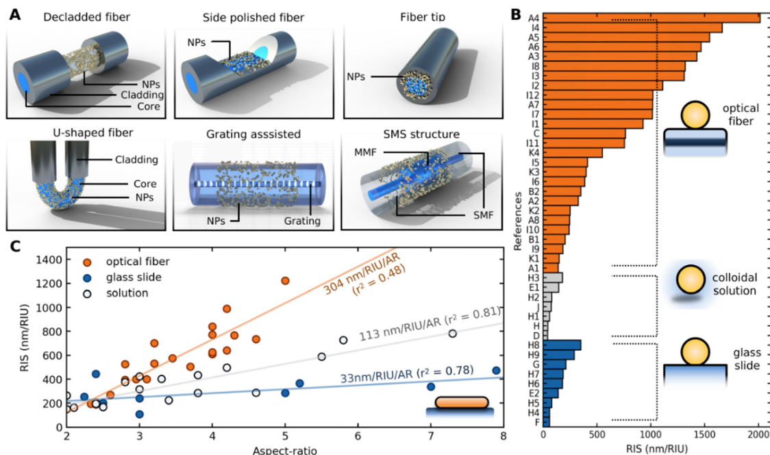
Fig. 27 (A) Typical nanoparticle-based plasmonic optical fiber sensor configurations (B) Refractive index sensitivity (RIS) comparison between Au nanospheres (NSs) immobilized on optical fiber sensor configurations, glass slides, or in colloidal solutions. The data labels correspond to the following works: A1-A8; 718 B1,B2; 739 C; 716 D; 736 E1,E2; 734 F; 740 G; 741 H; 742 H1-H9; 719 I1-I12; 720 J; 743 (C) RIS for gold nanorods (NRs) comparison for the same two optical platforms and on colloidal solution. Data were reproduced from ref. 678, 724, 732, 736, 738, 740, 742, 744–748 with permission from ACS publication, Springer New York publisher, ACS publication Elsevier publisher, MDPI publisher, Copyright 2007, 2022, 2016, 2008, 2022, 2007, 2009, 2021, 2018 respectively.
