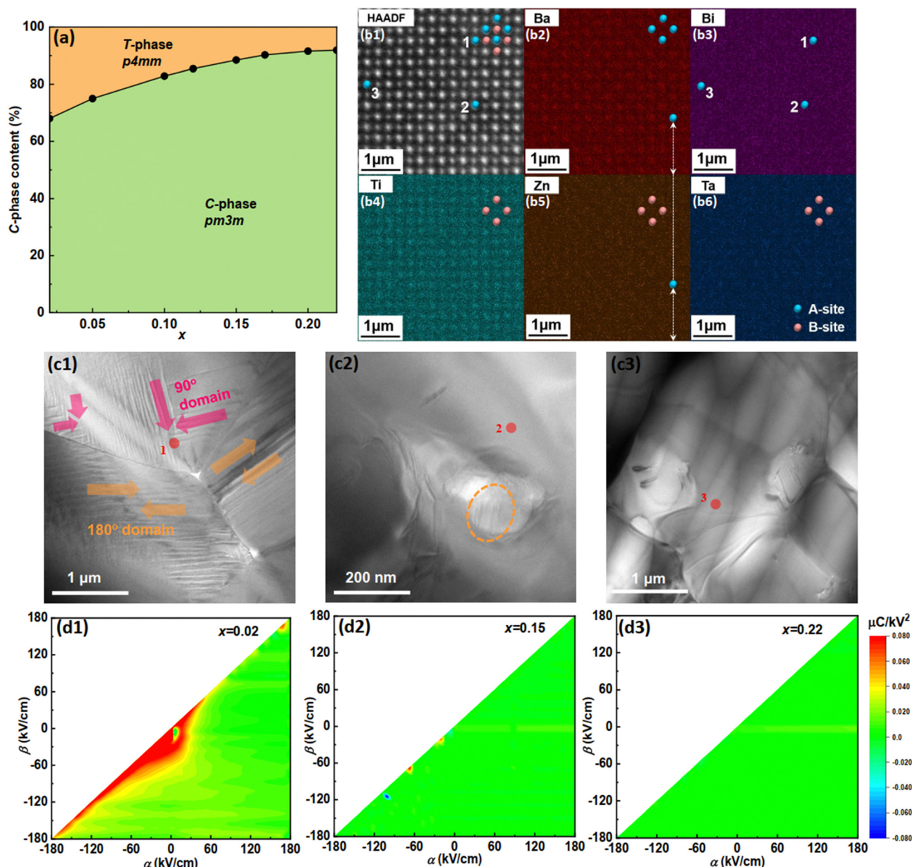
Fig. 1 (a) Phase diagram of BCZT- x BZT with x = 0.02 – 0.22 ; (b1) HAADF image of BCZT-0.15BZT; (b2)–(b6) atomic-EDS mapping for Ba, Bi, Ti, Zn, and Ta of BCZT-0.15BZT; (c1)–(c3) TEM image; (d1)–(d3) the FORC diagram of BCZT- x BZT with x = 0.02 , 0.15 , and 0.22 .
