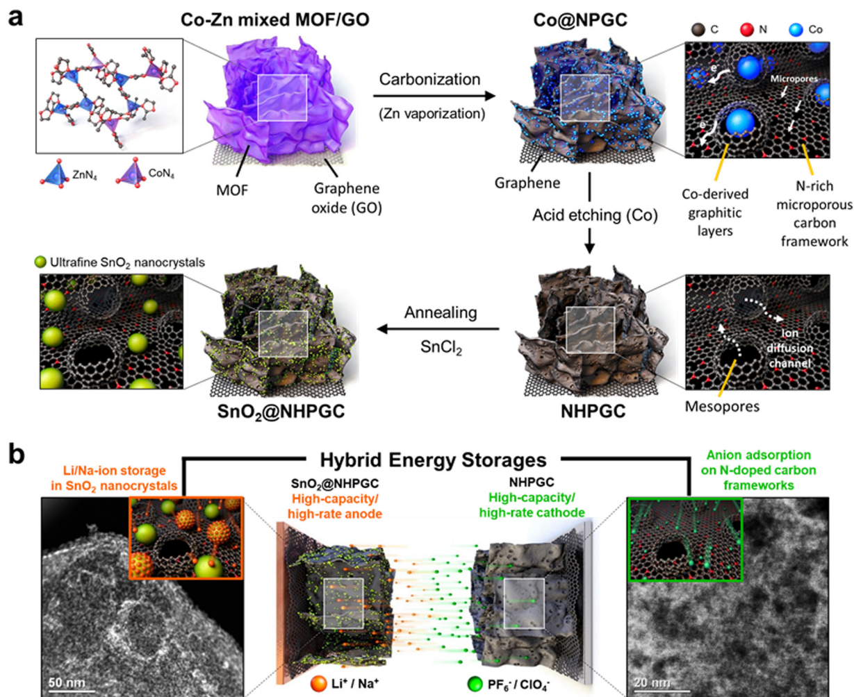
Fig. 1 A schematic illustration of synthesis processes and hybrid energy storage configuration. (a) Synthesis processes for NHPGC materials from Co–Zn mixed bimetallic MOFs on GO sheets and SnO_2@NHPGC with ultrafine SnO_2 nanocrystals integrated into NHPGC. (b) The hybrid energy storage configuration with the high-capacity/high-rate NHPGC cathode and SnO_2@NHPGC anode.
