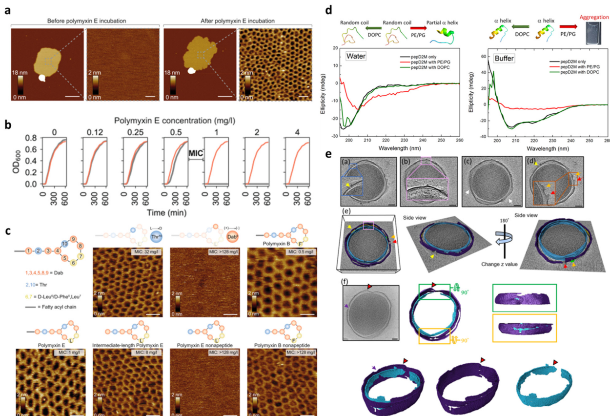
Fig. 9 a) AFM topographs of an OM patch before and after incubation with polyxymins E. Scale bars, 200 nm (overview) and 20 nm (zoom-in). b) Growth curves of the E. coli MG1655 WT (gray) and MG1655MCR-1 (red) strains at different polyxymins E concentrations. Above the minimal inhibitory concentration (MIC) of 0.5–1 mg L -1 , the growth of the E. coli MG1655 WT strain is inhibited. c) Schematic representation of the polyxymins structure, where polyxymins E has D-Leu (L) and polyxymins B has D-Phe (F) in the 6th position and AFM topographs of OM patches from the E. coli MG1655 WT strain upon incubation with different polyxymins E and polyxymins B variants (50 mg L -1 ). Crystalline structures are formed with the enantiomer variant Thr10 (L → D) and with full and intermediate-length polyxymins E variants. Structures are not formed in the polyxymins variant Dab9 (+) → (-) and polyxymins E nonapeptide variant. With polyxymins B variants, crystalline structures are formed in all cases. Panels a–c are reproduced and adapted with permission under a Creative Commons License (CC-BY 4.0) from ref. 146. Copyright © 2022 Springer Nature. d) CD spectra of pepD2M in water and in buffer. Black line: without liposomes; red line: mixed with PE/PG liposomes; green line: mixed with DOPC liposomes. Illustrations of the structural change that occurs upon conditional changes are shown above the spectra. e) Cryo-ET slices of two minicells treated with pepD2M and their inner and outer membranes. IM: cyan; OM: violet; PG: yellow; released material: green. Scale bar = 100 nm. Pores are pointed by arrows with different colors. Two volcanic-crater-like pores are indicated by the red and orange arrows. Panels d and e are reproduced and adapted with permission under a Creative Commons License (CC-BY 4.0) from ref. 147. Copyright © 2023 Springer Nature.
