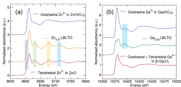
Fig. 4 (a) XANES region of the XAS data measured on the Zn K-edge for Li_{5.25}Zn_{0.37}BaLa_2Ta_2O_{12} and Zn(NO_3)_2 \cdot 6H_2O and ZnO standards. (b) XANES region of the XAS data measured on the Ga K-edge for Li_{5.25}Ga_{0.25}BaLa_2Ta_2O_{12} and Ga(NO_3)_3 \cdot 9H_2O and Ga_2O_3 standards. Coloured boxes indicate common features in the XANES profiles between the different materials analysed.
