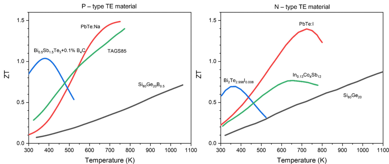
Fig. 7 Relationships between zT and optimal operating temperature ranges for selected TE materials. On the left-hand side, p-type materials include B-doped SiGe, 31 PbTe:Na, 30 Bi 0.5 Sb 1.5 Te 3 + 0.1B 4 C, 36 and TAGS85. 37 On the right-hand side, n-type materials feature SiGe, 38 PbTe:I, 32 Bi 2 Te 2.998 I 0.008 , 35 In-filled CoSb 3 . 39,40
