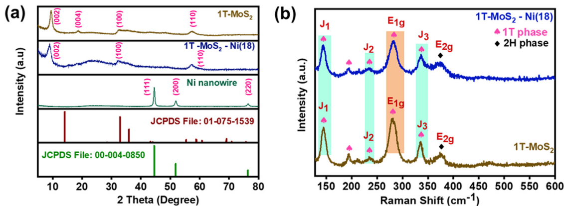
Fig. 2 (a) XRD patterns of the Ni nanowire, 1T-MoS 2 and 1T-MoS 2 -Ni(18) as compared with the standard patterns of MoS 2 (JCPDS File No. 01-075-1539) and metallic Ni (JCPDS File No. 00-004-0850). (b) Raman spectra of the as-synthesized 1T-MoS 2 and 1T-MoS 2 -Ni(18) composite material.
