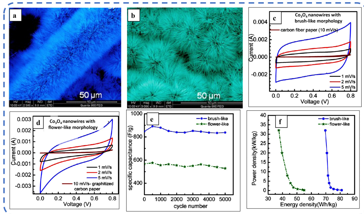
Fig. 18 (a) and (b) SEM images of \text{Co}_3\text{O}_4 -b and \text{Co}_3\text{O}_4 -f nanowires. (c) and (d) CV, (e) cycle stability and (f) Ragone plot of brush-like ( \text{Co}_3\text{O}_4 -b) and flower-like ( \text{Co}_3\text{O}_4 -f) nanowires. Reproduced with permission from ref. 181. Copyright 2012 ACS Publications.
