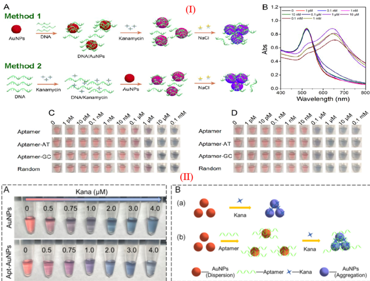
Fig. 6 (I) (A) Different approaches used for colorimetric assays of KANA, (B) Absorption spectra of AuNPs in presence of KANA. Colorimetric change of AuNPs after treating with the aptamer with increasing concentration of KANA in the (C) absence and (D) presence of NaCl with different aptamer. [Reproduced from ref. 93 with permission from [American Chemical Society], copyright [2020]]. (II) (A) color change of AuNPs in the presence of KANA without and with the presence of aptamer. (B) systematic representation of colorimetric aptasensor for KANA [Reproduced from ref. 94 with permission from [Elsevier], copyright [2022]].
