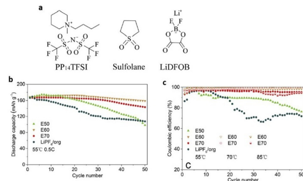
Fig. 10 (a) Chemical structures of 1-methyl-1-butylpiperidinium bis(trifluoromethanesulfonyl)-imide (PP 14 TFSI), sulfolane and lithium difluoro(oxalato)borate (LiDFOB). (b) and (c) Cycling stability and coulombic efficiency and rate performance of Li/Li-rich half cells at 55 and 70 ^\circ\text{C} at 0.5C and 85 ^\circ\text{C} at 1C under a voltage range of 2.0–4.6 V. Reproduced from ref. 79 with permission from Elsevier, Copyright [2018].
