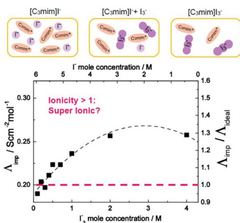
Fig. 5 Molar conductivity ( \Delta_{imp} ) and ionicity ( \Delta_{imp}/\Delta_{ideal} ) of [C_3mim]I^- with added I_3^- as a function of I_3^- ( I^- ) concentration at iso-viscosity state of 0.2 Pa s. Reproduced from ref. 65 with permission from RSC, Copyright [2018].
