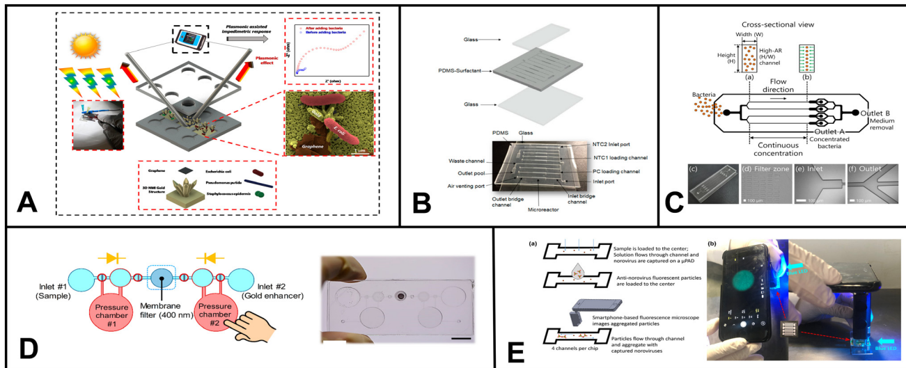
Fig. 3 Examples of microfluidic devices for microorganism detection in water. (A) Optoelectrical detection platform for bacteria based on plasmon-assisted electrochemical impedance spectroscopy (PEIS). The microfluidic device consists of 3D gold nano/microislands (NMIs) and graphene nanosheets (adapted from ref. 191 with permission, copyright 2020, American Chemical Society). (B) Microfluidic array chip using PCR-based detection of waterborne bacteria (reprinted from ref. 192). (C) Schematic illustrating the process of continuous bacterial concentration using viscoelastic fluid. (a) Bacteria dispersed in a viscoelastic fluid are introduced randomly at the inlet. (b) Elastic forces cause bacterial cells to concentrate at the center of the microchannel. At the outlet, tightly focused cells are collected at the central outlet (outlet A), while the suspending medium is directed to the side outlets (outlet B). (c) Image depicting the fabricated device employed in this study for bacterial concentration. Microscopic images of (d) the filter zone, (e) the inlet, and (f) the outlet region of the microchannel (reprinted from ref. 189). (D) Colorimetric-based device using immunomagnetic separation to detect E. coli (reprinted from ref. 193). (E) Paper-based device coupled with smartphone technology for fluorescent detection of norovirus in environmental water samples. The figure schematic illustrates (a) the introduction of norovirus solutions and anti-norovirus particle suspension, and (b) the application of Blue LED irradiation to the \mu PAD from the side (reprinted from ref. 186 with permission, copyright 2019, American Chemical Society, https://pubs.acs.org/doi/10.1021/acsomega.9b00772 , further permission related to the material excerpted should be directed to the ACS).
