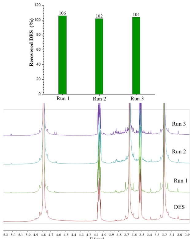
Fig. 7 Yields (top) and 1 H-NMR (bottom) of the recovered DES after each cycle.
