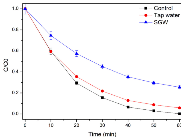
Fig. 10 Degradation of CIP in real water matrix, experimental conditions: [CIP] = 1 ppm, TP = 1% TiO_2 , 0.7% PVP with PVDF beads, volume: 50 mL.
