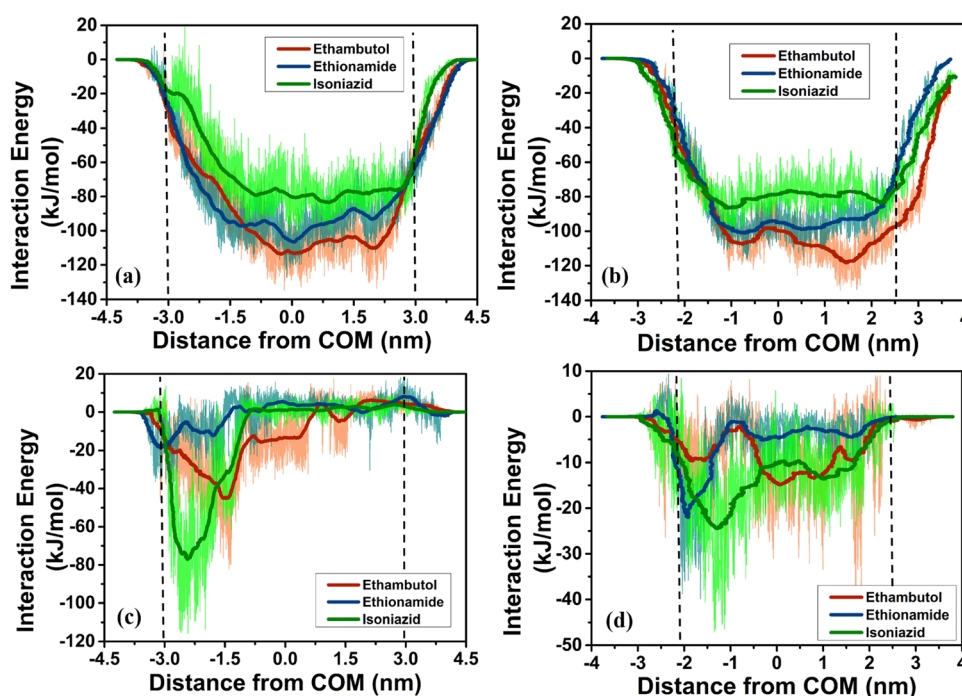
Fig. 2 Different modes of drug–monolayer interaction during the pulling of drug molecules through the monolayer. Spatial variation of drug–membrane vdW interaction energy during the passage of drugs through the MA monolayer for (a) CHARMM and (b) GROMOS FFs. Positional dependency of electrostatic interactions for (c) CHARMM and (d) GROMOS FFs. In the figures, vertical black dashed lines represent positions of water–monolayer interfaces.
