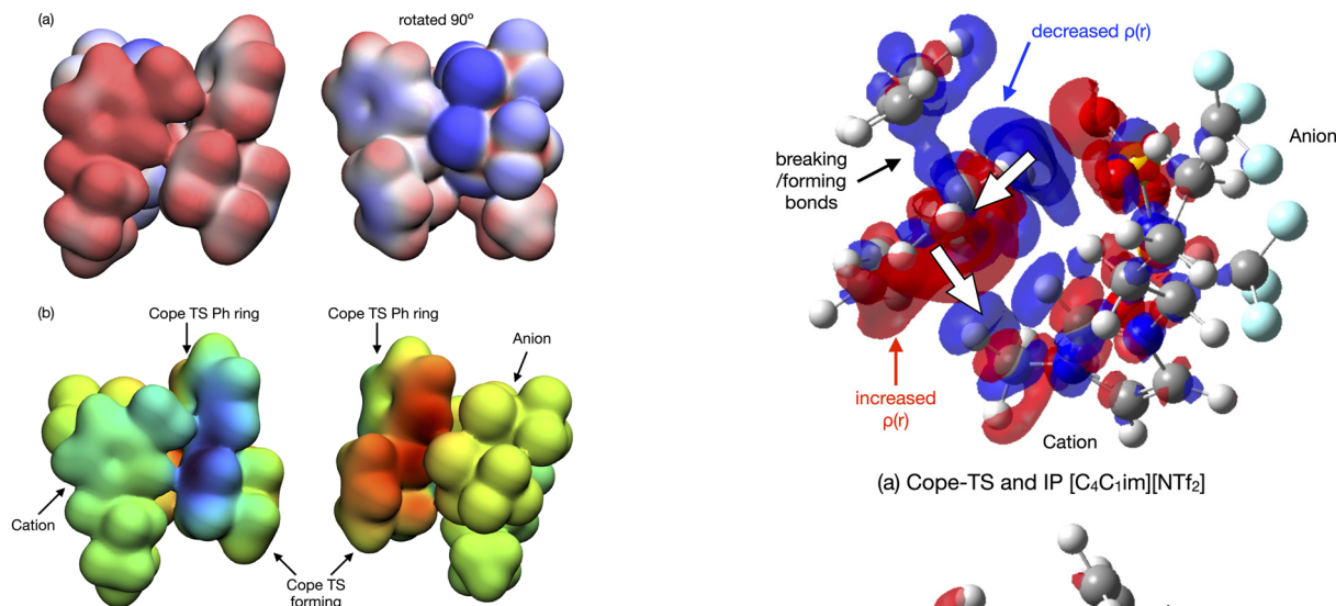
Fig. 13 Reaction B TS-[C 4 C 1 C 1 im][NTf 2 ] (a) electrostatic potential (ESP) mapped onto the 0.007 density iso-surface, red positive, blue negative, maximum \pm 0.05 a.u., (b) \Delta\rho = \rho_{\text{cluster}} - (\rho_{\text{TS}} + \rho_{\text{solvent}}) mapped onto the 0.007 a.u. ( e/a_0^3 ) density iso-surface. "Rainbow" colour scheme, blue = negative, green = neutral, red = positive, maximum \pm 0.02 a.u.
