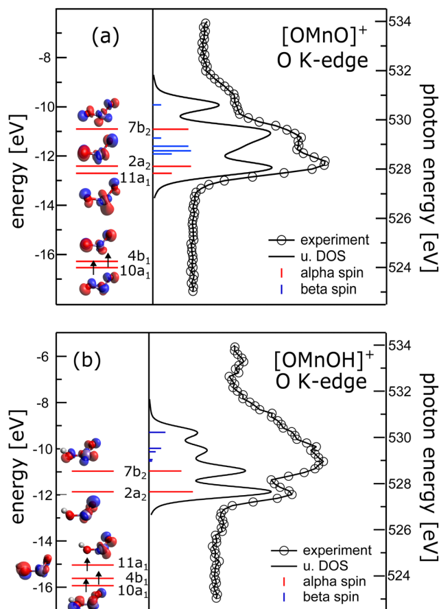
Fig. 2 Left panels: Energy level diagram deduced from \alpha spins along isosurface plots of the molecular orbitals of (a) [\text{OMn}^{\text{VO}}]^+ and (b) [\text{OMn}^{\text{VOH}}]^+ complexes. Arrows indicate occupied molecular orbitals. Right panel: Comparison of oxygen K-edge absorption (340 meV energy resolution) and oxygen p -projected density of states (broadened with a Gaussian of 0.3 eV full width half maximum and a 0.16 eV Lorentzian 49 to account for experimental resolution and core hole lifetime, respectively) of (a) [\text{OMn}^{\text{VO}}]^+ and (b) [\text{OMn}^{\text{VOH}}]^+ complexes. Blue and red sticks show \alpha and \beta spin states, respectively. For [\text{OMn}^{\text{VOH}}]^+ we use the molecular orbital nomenclature in C_{2v} symmetry as the local symmetry at the metal is only slightly disturbed by the addition of the hydrogen atom. This allows for a more direct comparison to [\text{OMn}^{\text{VO}}]^+ .
