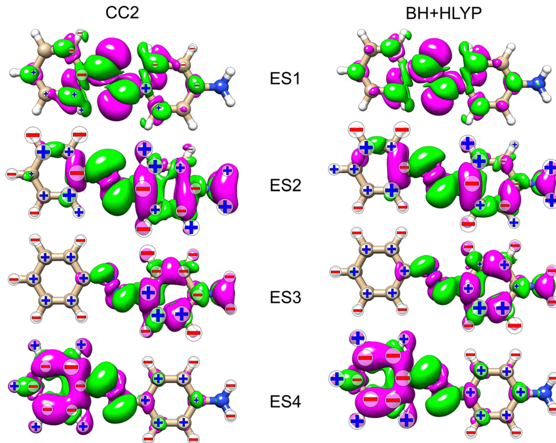
Fig. 9 AZO-2. RI-CC2 and TD-DFT/BH+HLYP (aug-cc-pwCVDZ basis set) difference densities for the four lowest excited states (ES) with the sign (+/–) of the nuclei's \mathcal{L}_K\mathcal{B}_K terms. The size of the sign indicates the magnitude (magnified by 1000) of the signal (smallest for 1 < |\text{NSCD}| < 10 , middle size for 10 < |\text{NSCD}| < 100 and largest for |\text{NSCD}| > 100 . NSCD signals with absolute values < 1 are not shown).
