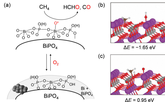
Fig. 14 (a) Proposed mechanism for CH 4 oxidation over BiPO 4 catalyst. DFT calculation for H abstraction from CH 4 by (b) the O atom adsorbed on surface Bi and (c) the lattice O atom. (Reproduced from ref. 52 with permission from Royal Society of Chemistry).
