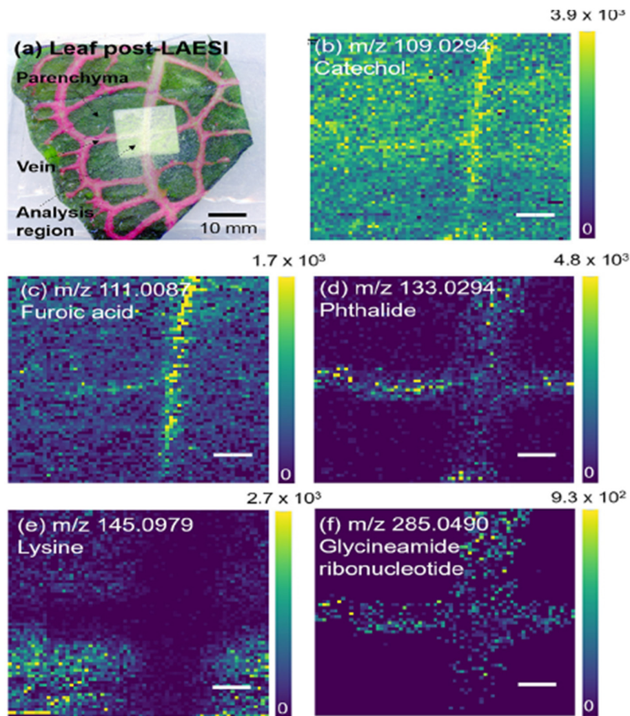
Fig. 9 LAESI-MSI of F. argyoneura leaf in high spatial resolution (40 \mu\text{m} ) in negative ion mode. (a) Optical image of leaf post-LAESI imaging showing analysis region (lighter region). Single ion images (b–f): (b) catechol (vein), (c) furoic acid (vein), (d) phthalide (vein), (e) lysine (parenchyma), (f) glycineamide ribonucleotide (vein). Color bars shown as signal/noise, and scale bars are 200 \mu\text{m} . Reprinted (adapted) from ref. 1 with permission from American Chemical Society, copyright. 1
