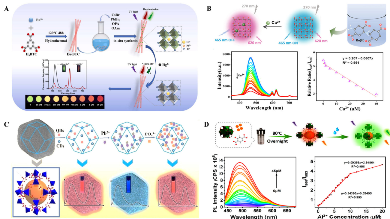
Fig. 7 Ion sensing of MOF-based ratiometric fluorescent probes. (A) Schematic diagram of the synthesis process of \text{CsPbBr}_3@Eu\text{-BTC} and the ratiometric fluorescence sensing of \text{Hg}^{2+} . 77 (B) Schematic diagram of ratiometric fluorescence sensing of \text{Cu}^{2+} in serum by \text{Eu-DATA/BDC} . 78 (C) Schematic diagram of \text{CDs/QDs@ZIF-8} for ratiometric fluorescence sensing of \text{Pb}^{2+} and \text{PO}_4^{3-} . 79 (D) Schematic diagram of the preparation of \text{UiO(OH)}_2@RhB and the sensing process for \text{Al}^{3+} . 80
