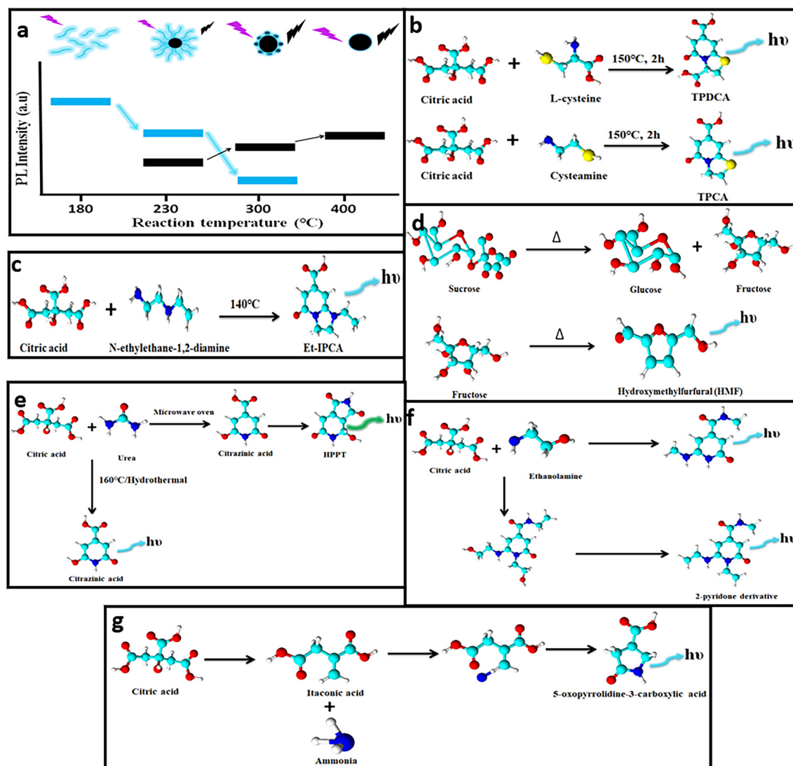
Fig. 3 (a) Emission intensity of CDs using citric acid and ethylenediamine as precursors during synthesis under different temperatures. 66 (b–f) Different types of molecular fluorophoric species 71,73–76 and (g) unconventional aliphatic fluorophores identified that contribute to the fluorescence of CDs. 77
