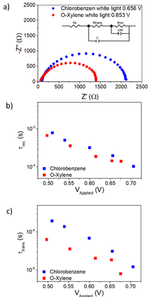
Fig. 5 (a) Nyquist spectra from impedance measurements of azatriangulene-based organic solar cells using o -xylene and chlorobenzene as solvents under white illumination. Equivalent circuit used to fit the resulting spectra included as inset. Recombination lifetime (b) and electron diffusion transit time (c) extracted from the impedance spectra of azatriangulene-based organic solar cells using o -xylene and chlorobenzene as solvents under white illumination, applying the equivalent circuit depicted in the inset of (a).
